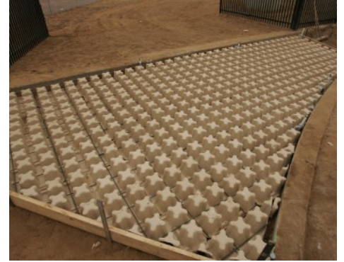
Grasscrete - Molded Pulp Former in Position
