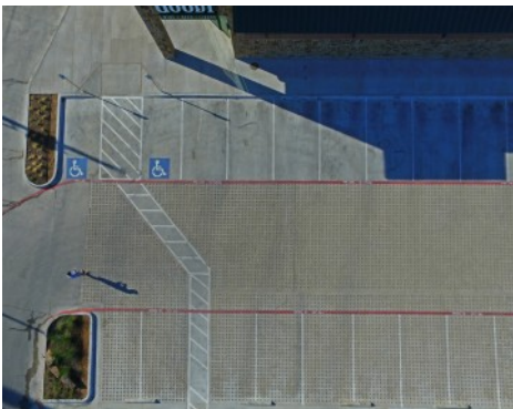
Goody Goody Liquor Store Parking Lot - Bomanite Pervious Grasscrete Stone Filled System - ADA Access
